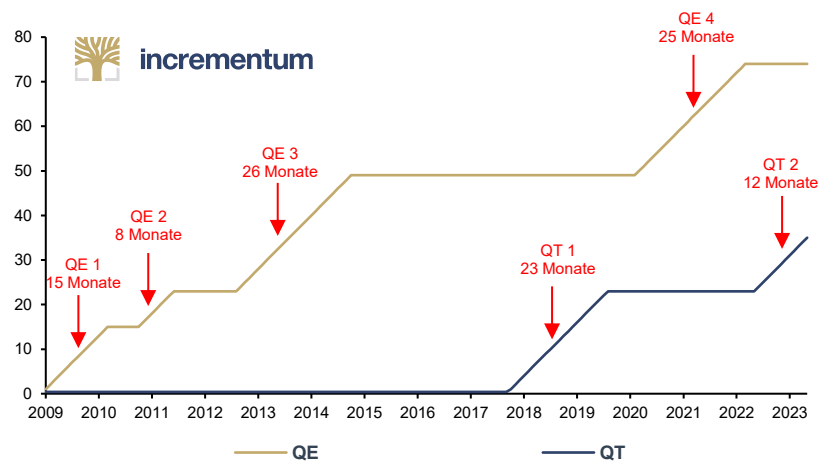
QE vs. QT, in Monaten, 01/2009-05/2023
