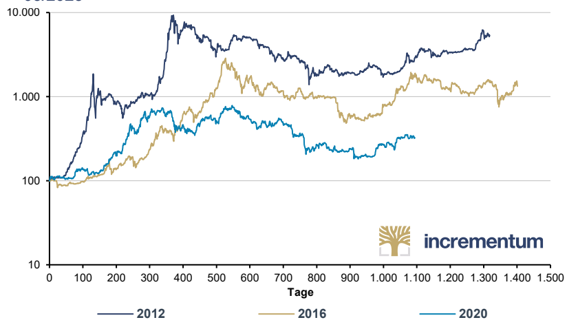
Bitcoin-Performance nach Halvings, 100 = Halving (log), 11/2012-05/2023
